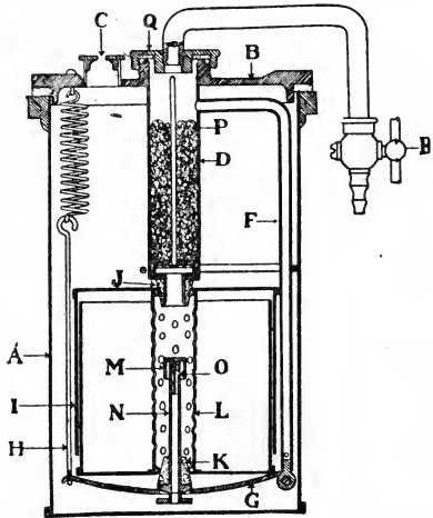
FIG. 6.—Signal lantern generator.
